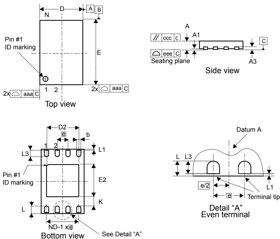
Figure 15. UFDFPN8 - Outline
