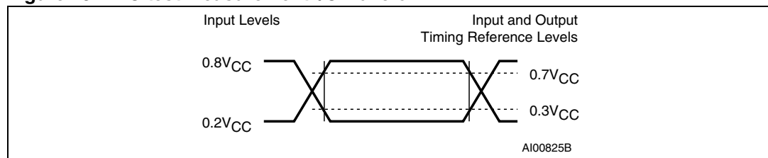
Figure 13. AC test measurement I/O waveform
