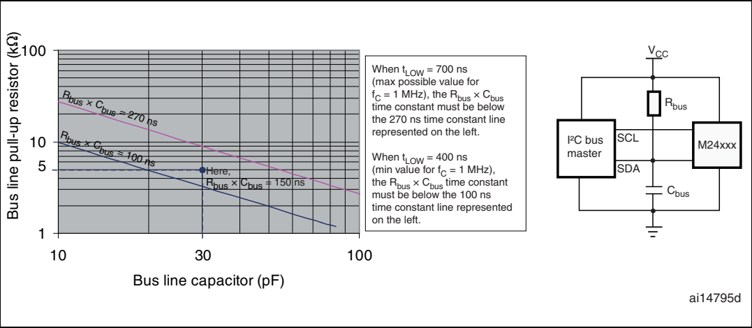
Figure 7. I 2 C Fast mode Plus ( f_C = 1\text{ MHz} ): maximum R_{bus} value versus bus parasitic capacitance ( C_{bus} )
