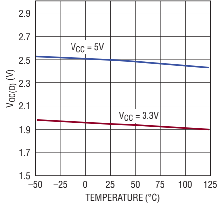
Common Mode Output Voltage (Dominant) vs Temperature
