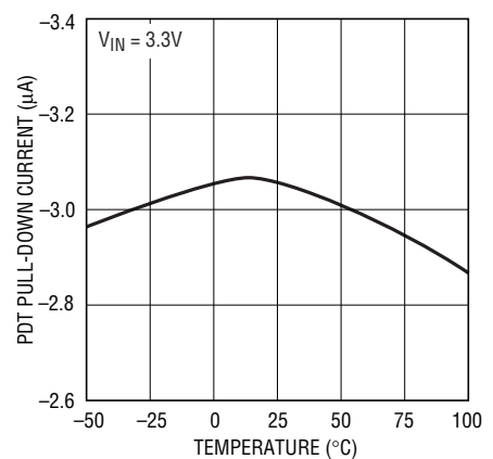
PDT Pull-Down Current vs Temperature
