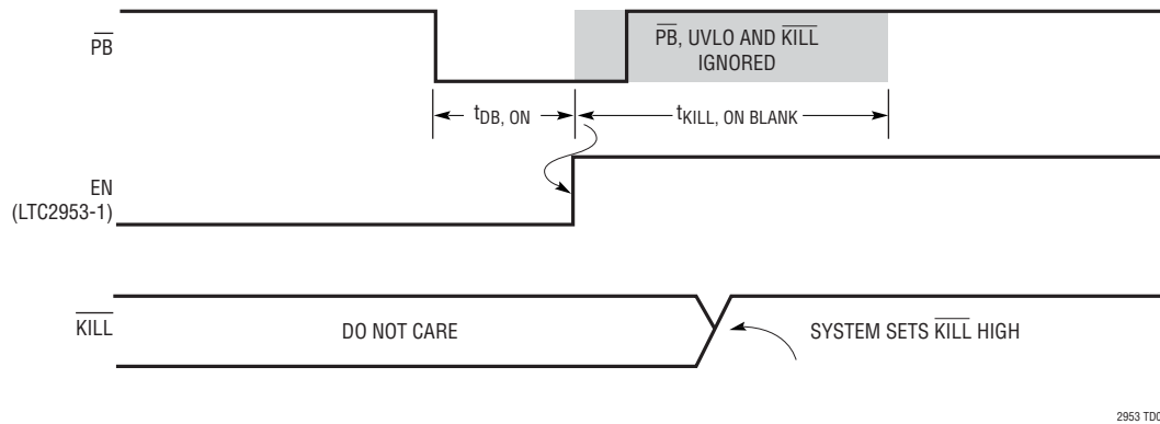
Figure 1. Power On Timing (UVLO &gt; 0.55V)
