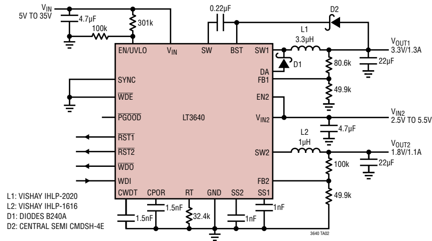
2MHz 3.3V/1.3A and 1.8V/1A Buck Regulators
