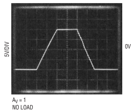
Large-Signal Transient Response V_S = \pm 15\text{V}
