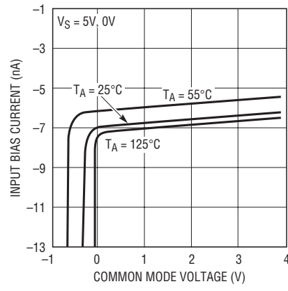
Input Bias Currents vs Common Mode Voltage
