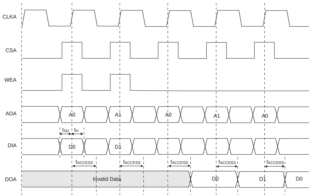
Figure 3-6. Read Mode
