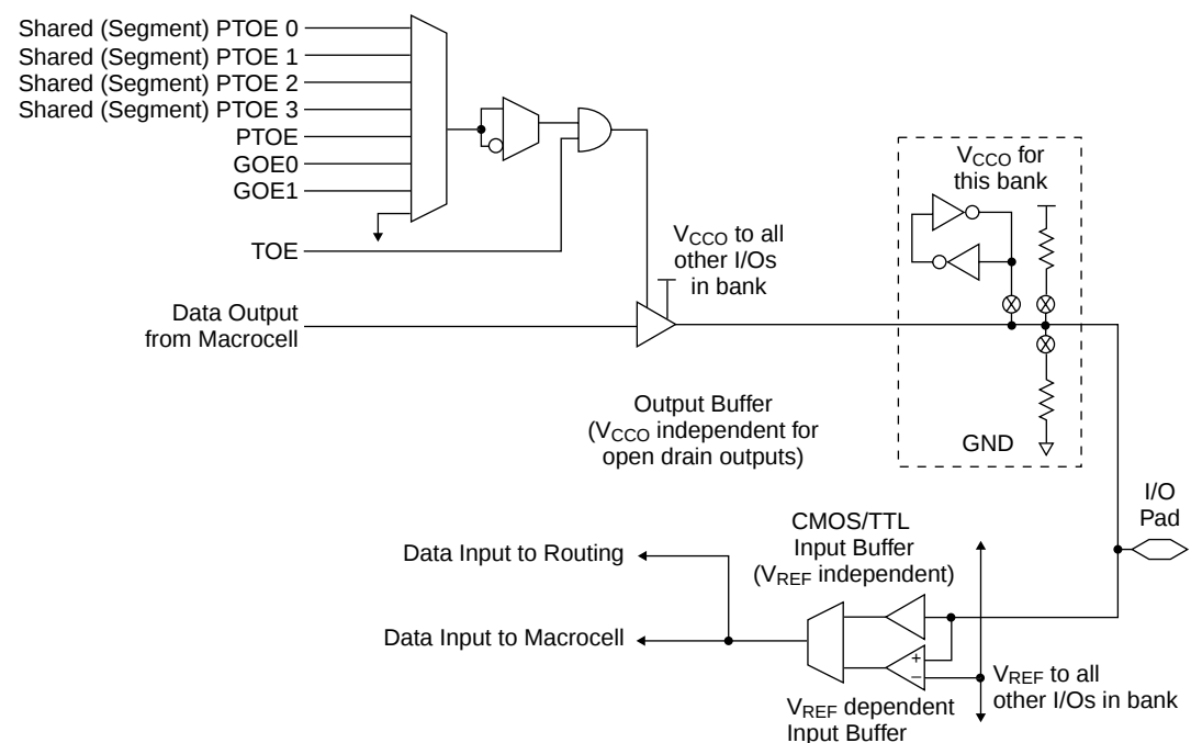
Figure 8. I/O Cell
