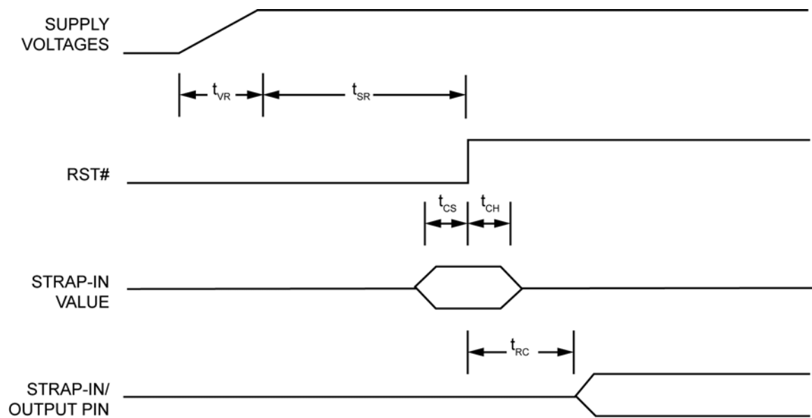
Figure 17. Power-Up/Reset Timing
