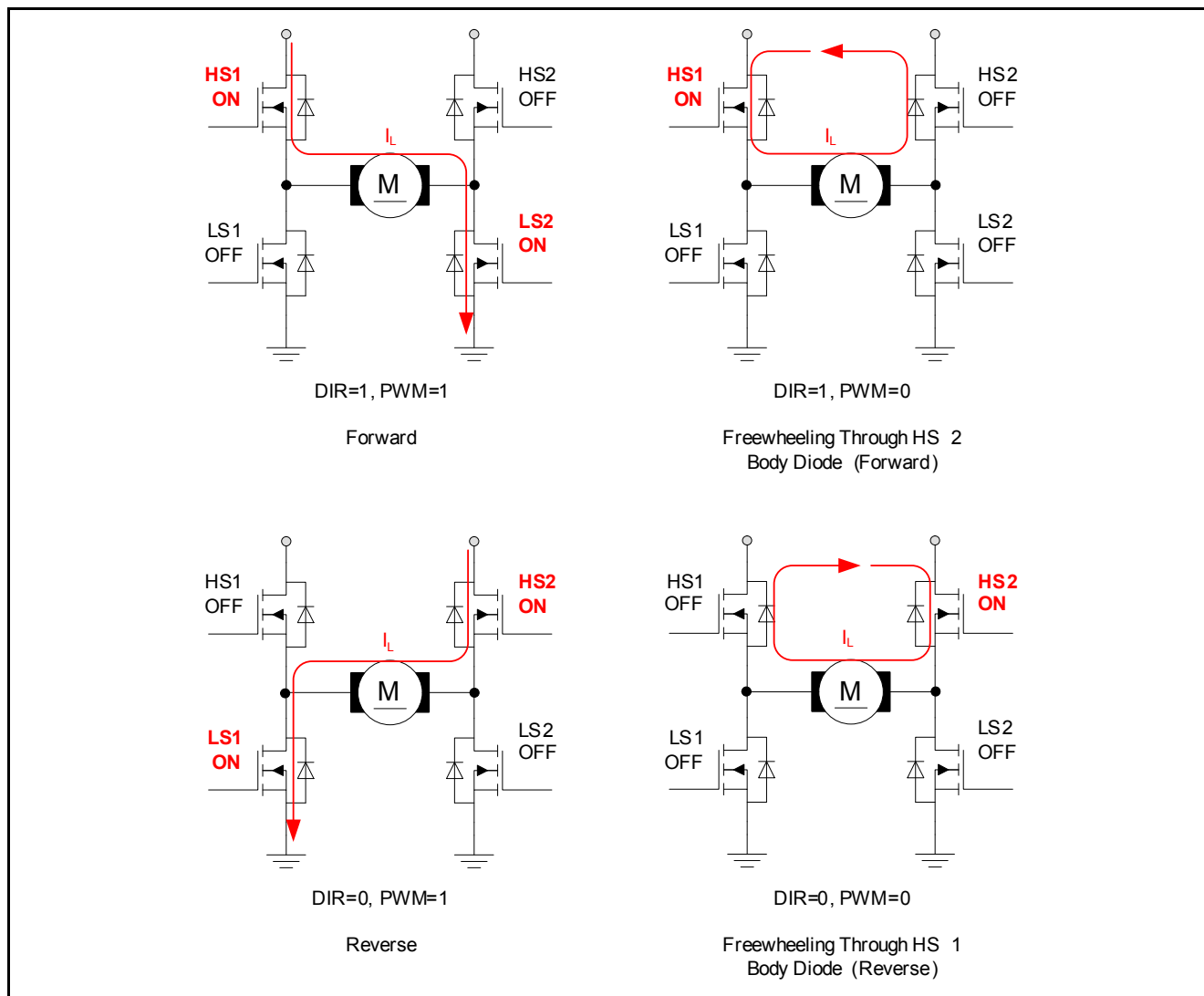
Figure 4-2 Operation Modes
