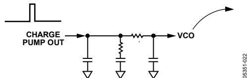
Figure 22. Typical Loop Filter Configuration
