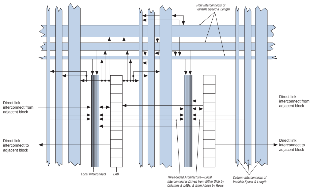
Figure 4-1. Stratix GX LAB Structure
