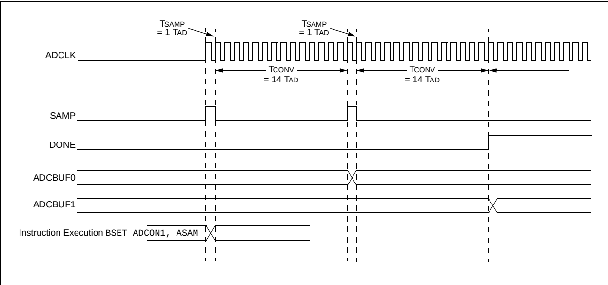
FIGURE 19-3: CONVERTING 1 CHANNEL AT 200 kps, AUTO-SAMPLE START, 1 TAD SAMPLING TIME
