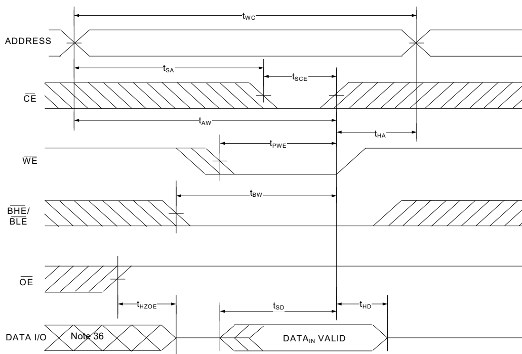
Figure 16. Write Cycle No. 1 ( \overline{\text{CE}} Controlled) [32, 33, 34]
