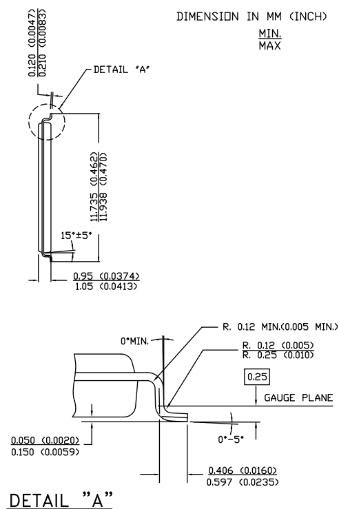
Figure 19. 54-pin TSOP II (22.4 × 11.84 × 1.0 mm) Package Outline, 51-85160
