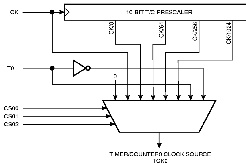
Figure 29. Timer/Counter0 Prescaler
