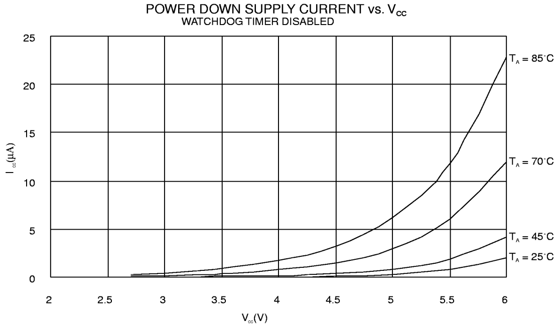
Figure 45. Power Down Supply Current vs. V_{CC}
