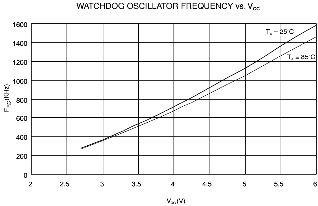
Figure 47. Watchdog Oscillator Frequency vs. V_{CC}
