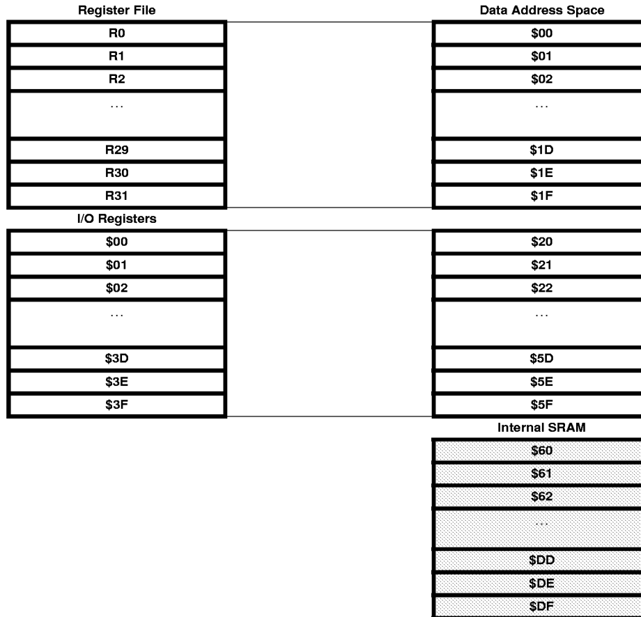
Figure 9. SRAM Organization
