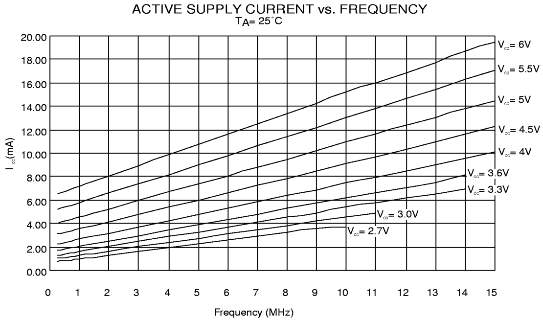
Figure 39. Active Supply Current vs. Frequency
