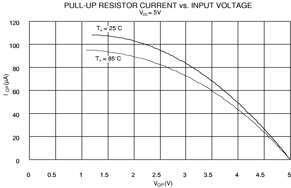
Figure 48. Pull-up Resistor Current vs. Input Voltage
