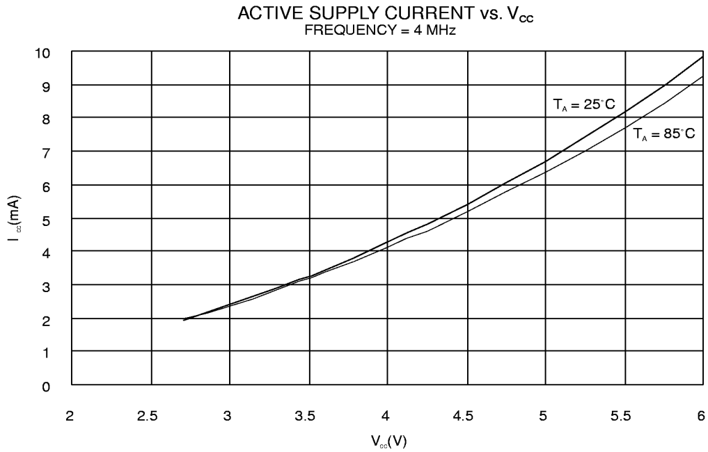
Figure 40. Active Supply Current vs. V_{CC}
