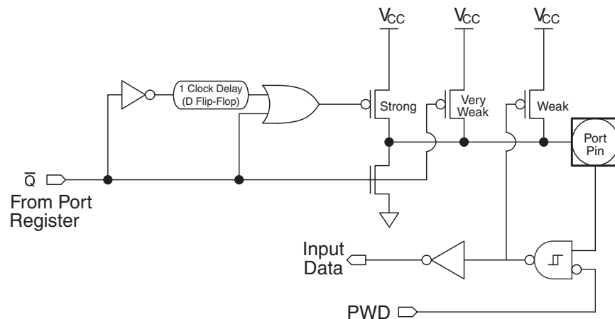
Figure 12-1. Quasi-bidirectional Output
