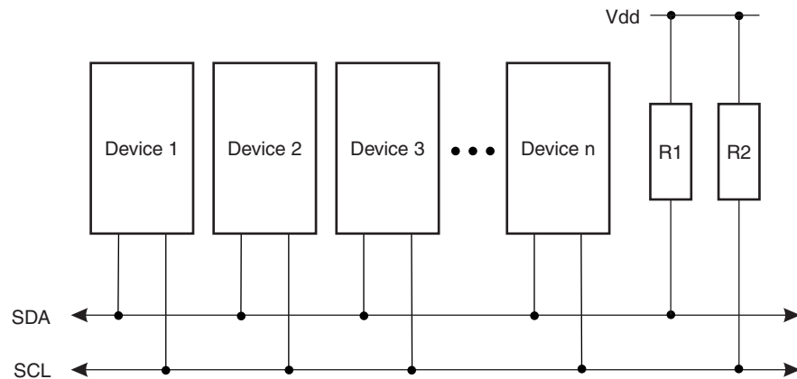
Figure A-1. I 2 C Interface Bus
