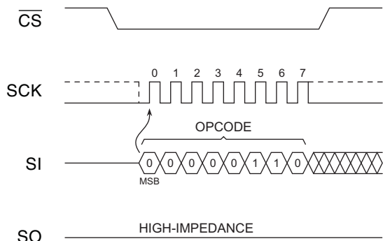
Figure 9-1. Write Enable
