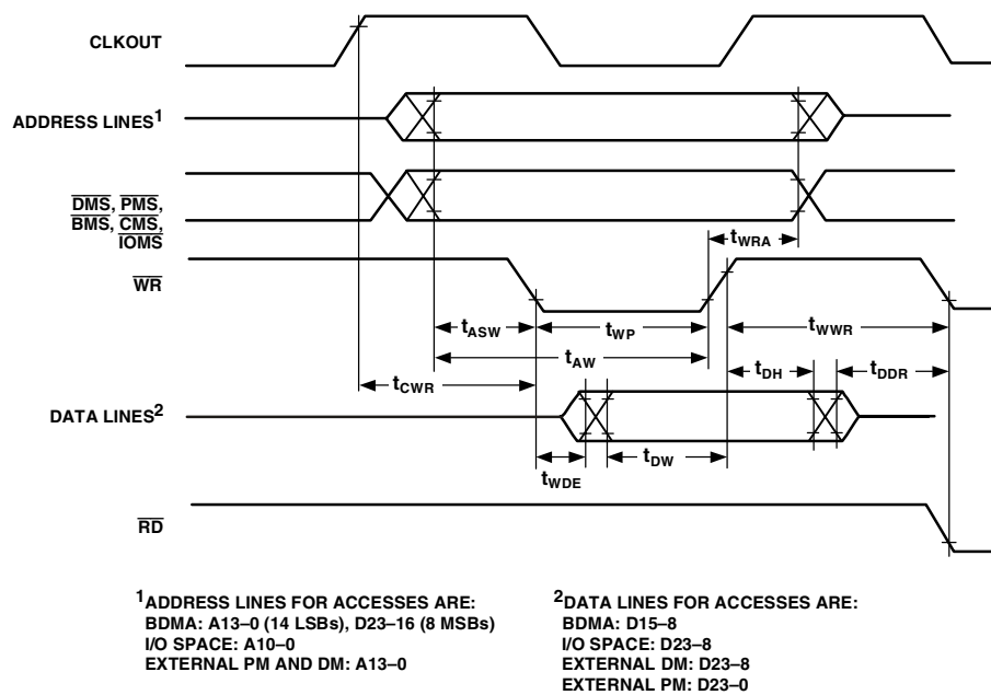
Figure 30. Memory Write
