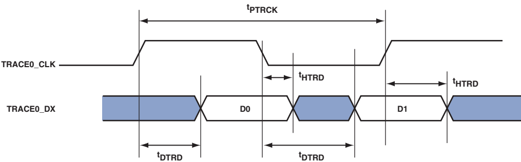
Figure 80. Trace Timing
