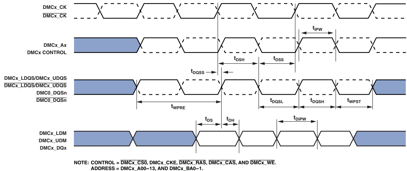
Figure 27. DDR3 SDRAM Controller Output AC Timing
