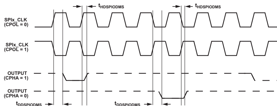
Figure 49. ODM Slave Mode
