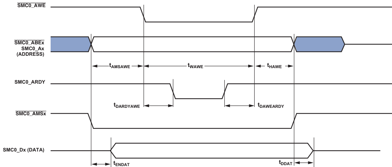
Figure 16. Asynchronous Write
