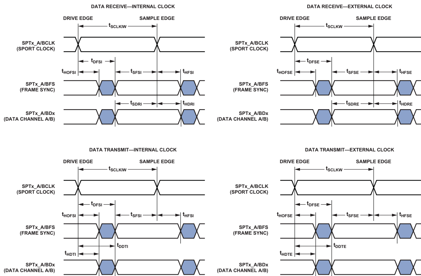
Figure 39. Serial Ports
