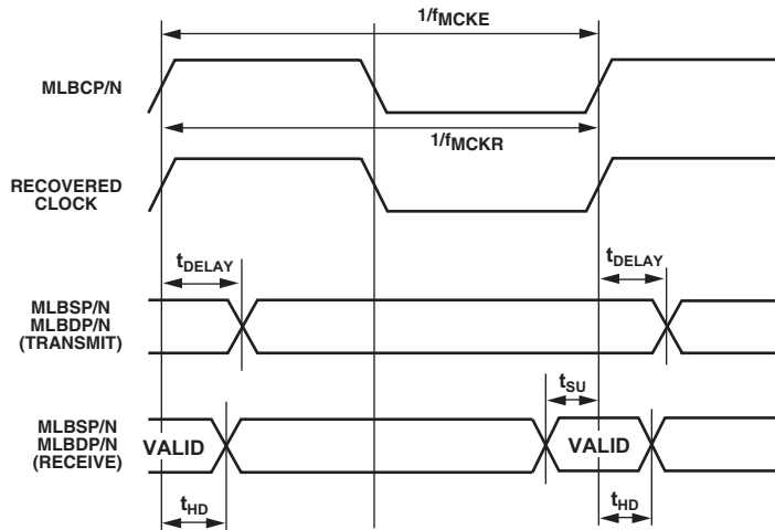
Figure 77. MLB 6-Pin Delay, Setup, and Hold Times
