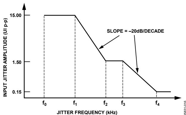
Figure 12. SONET Jitter Tolerance Mask
