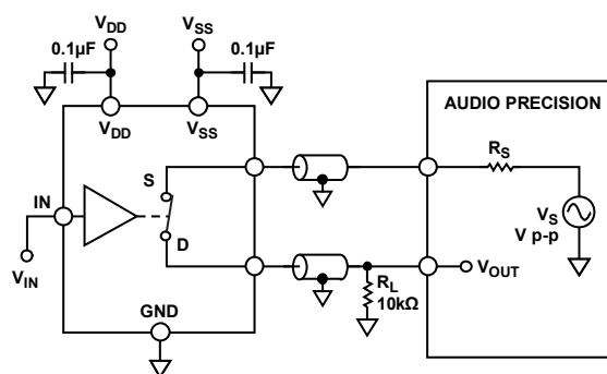
Figure 37. Channel-to-Channel Crosstalk
