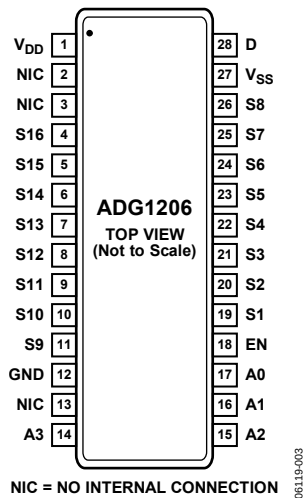
Figure 3. 28-Lead TSSOP Pin Configuration (ADG1206)
