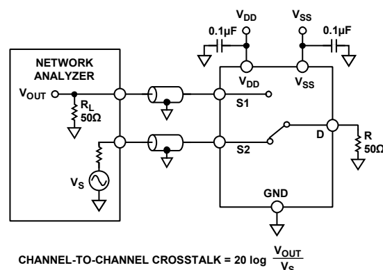
Figure 37. Channel-to-Channel Crosstalk
