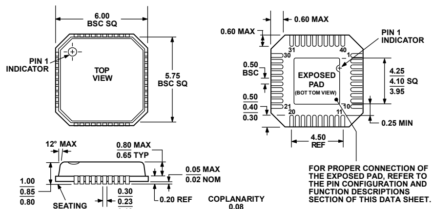
Figure 54. 40-Lead Lead Frame Chip Scale Package [LFCSP_VQ] 6 mm x 6 mm Body, Very Thin Quad (CP-40-1)
