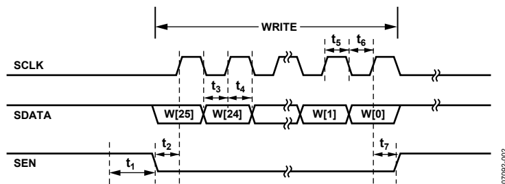
Figure 2. Serial Interface Write Diagram
