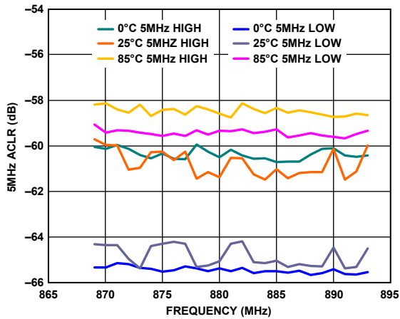
Figure 17. Transmit ACLR vs. Frequency and Temperature (UMTS Band V), Transmit Output Power = -7 dBm
