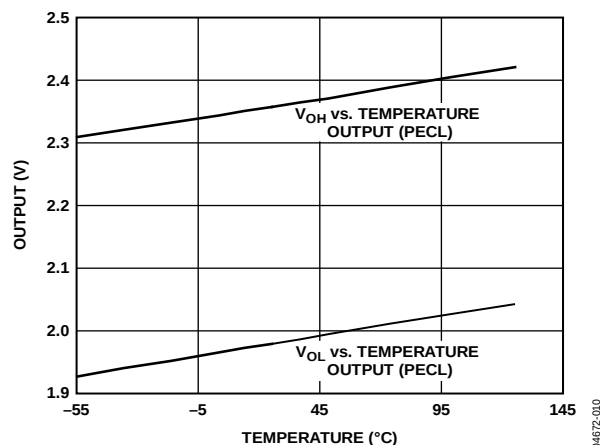
Figure 9. ADCMP582 Output Voltage vs. Temperature
