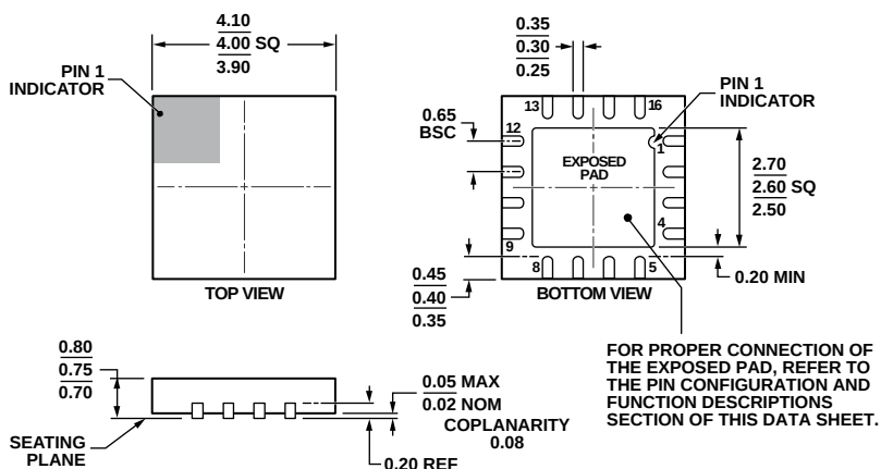
Figure 53. 16-Lead Lead Frame Chip Scale Package [LFCSP]
