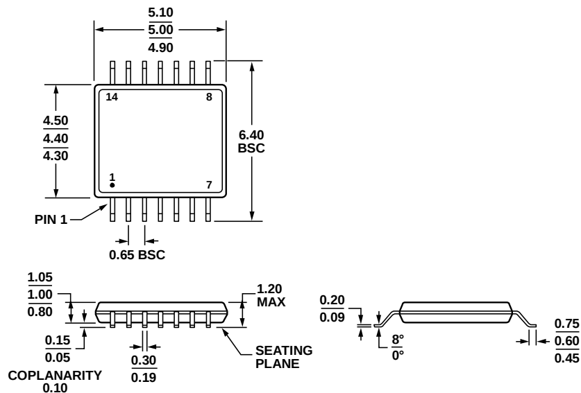
Figure 52. 14-Lead Thin Shrink Small Outline Package [TSSOP]
