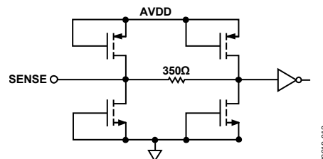
Figure 73. Equivalent SENSE Circuit
