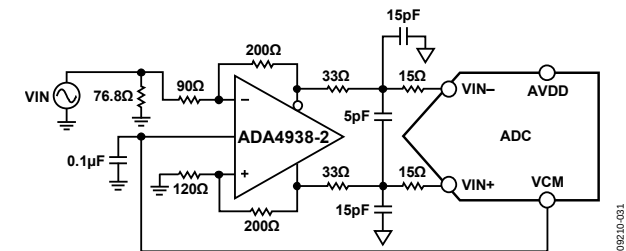
Figure 49. Differential Input Configuration Using the ADA4938-2
