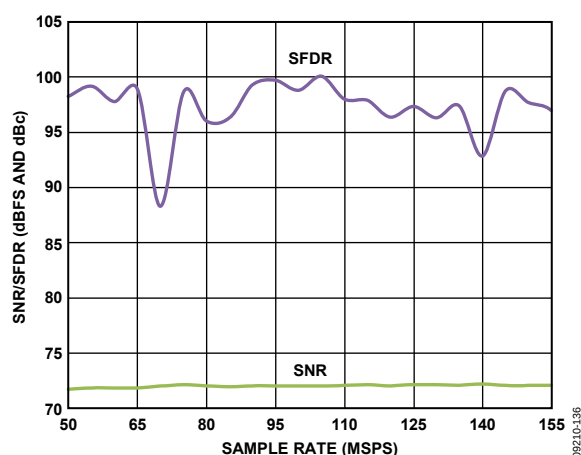
Figure 37. AD9641-155 Single-Tone SNR/SFDR vs. Sample Rate ( f_{IN} ) with f_{IN} = 70.1 MHz
