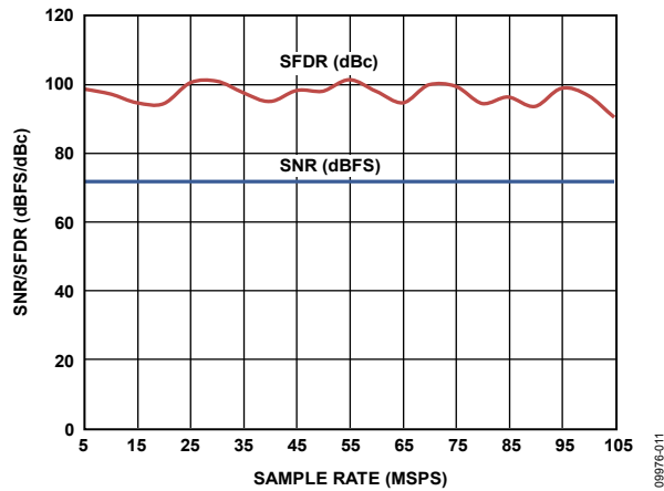
Figure 29. SNR/SFDR vs. Sample Rate with A_{IN} = 9.7 MHz
