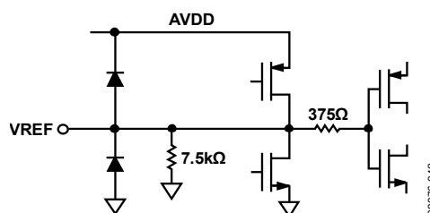
Figure 41. Equivalent VREF Circuit
