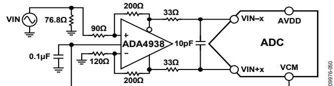
Figure 44. Differential Input Configuration Using the ADA4938-2
