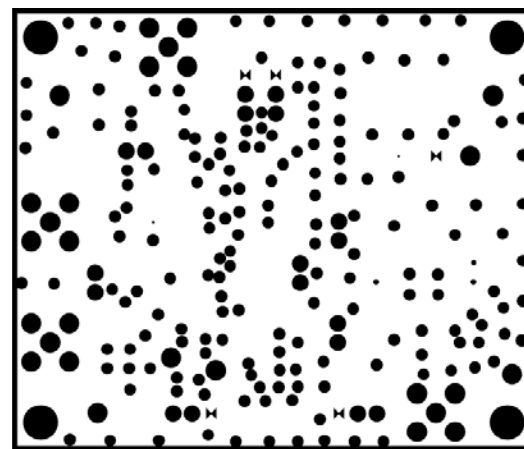
Figure 102. Power Plane
