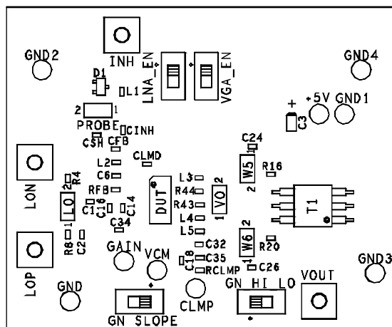
Figure 98. AD8331-EVALZ Assembly
