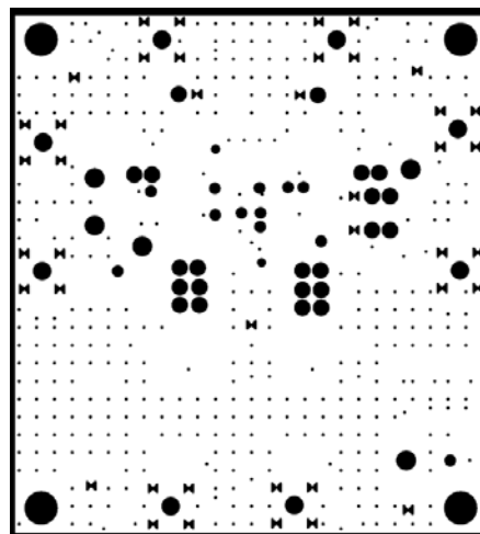
Figure 110. Ground Plane
