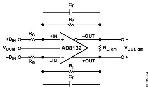
Figure 64. Circuit Definitions
