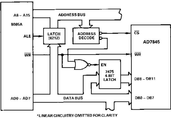
Figure 22. 8085A Interface
