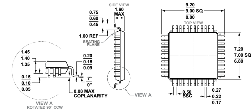
Figure 44. 48-Lead Low Profile Quad Flat Package [LQFP] (ST-48)
