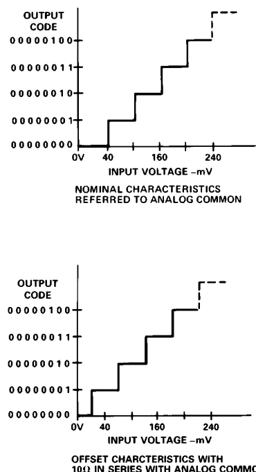
Figure 5. AD673 Transfer Curve—Unipolar Operation (Approximate Bit Weights Shown for Illustration, Nominal Bit Weights % 39.06 mV)
