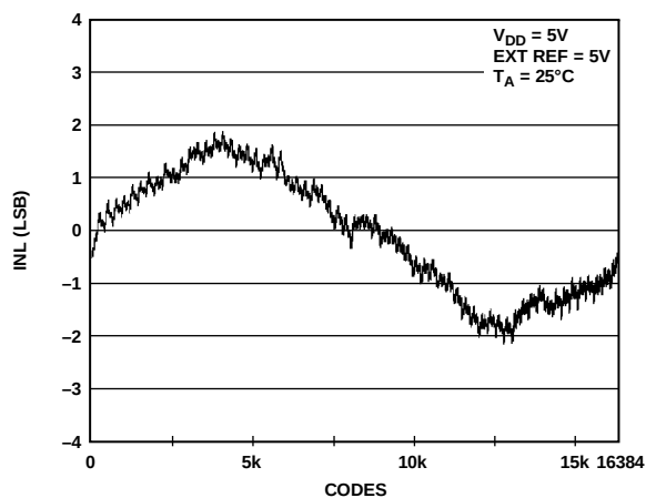
Figure 8. INL AD5648—External Reference
