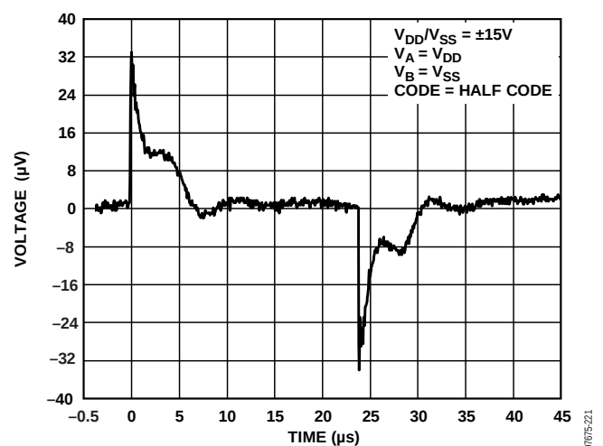
Figure 35. Digital Feedthrough
