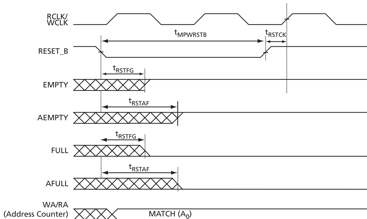
Figure 3-48 • FIFO Reset
