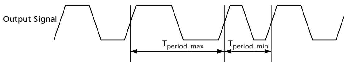
Figure 2-18 • Peak-to-Peak Jitter Definition
