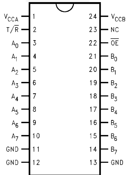
Figure 2. Pin Configuration
