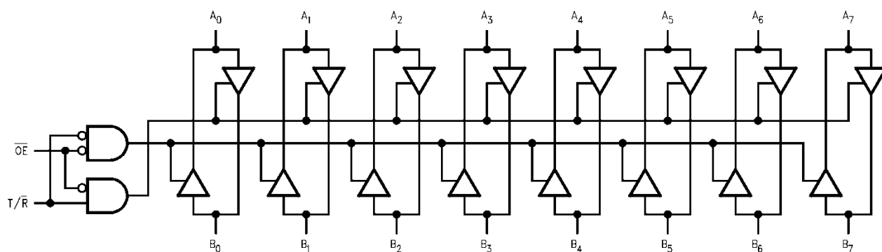
Figure 3. Logic Diagram
