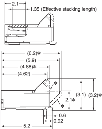
Applicable FPC/FFC Dimensions
