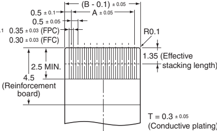
Applicable FPC/FFC Dimensions
