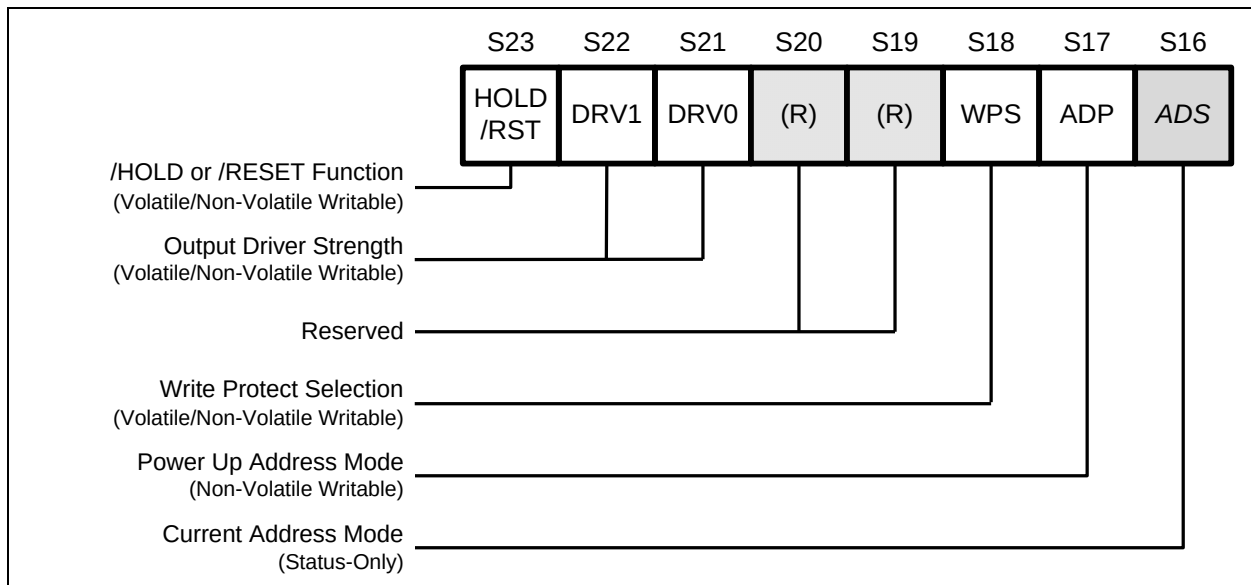
Figure 4c. Status Register-3
