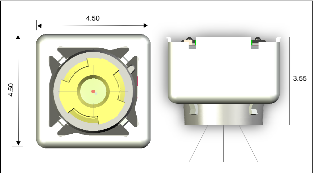
Figure 3. Module outline
