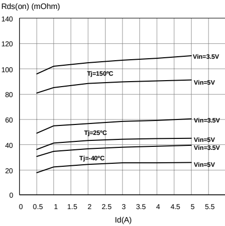
Figure 41. Static Drain-Source On resistance Vs. Input Voltage
