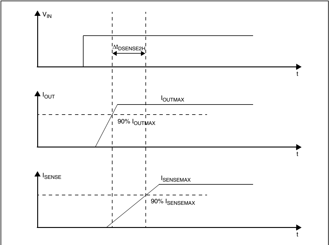
Figure 5. Delay response time between rising edge of ouput current and rising edge of current sense (CS enabled)
