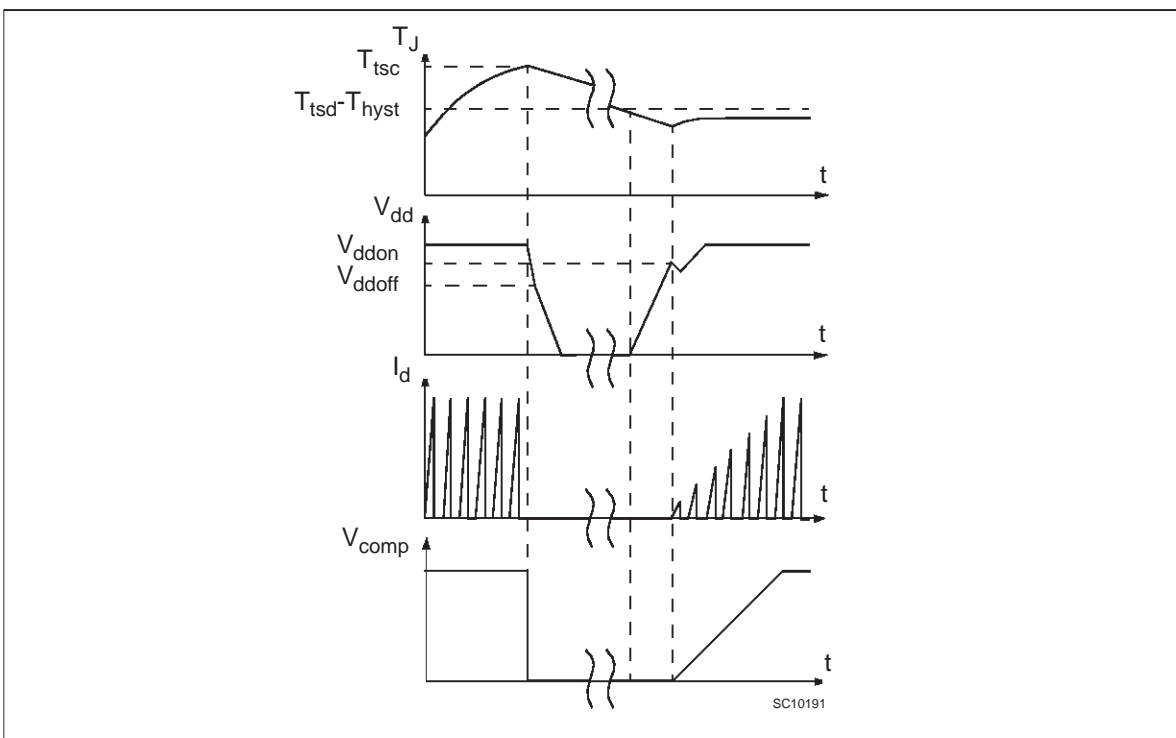
Figure 8: Overtemperature Protection
