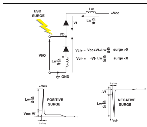
Figure 4. Surge behavior
