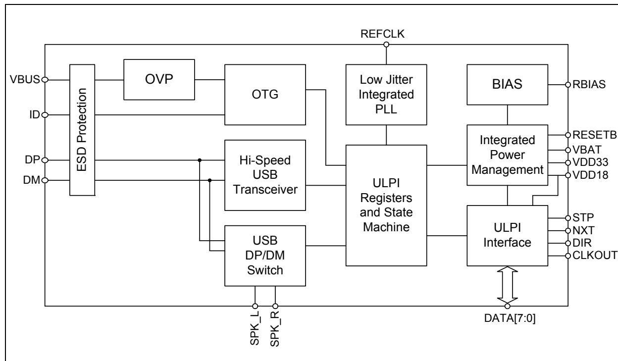
Figure 1 Block Diagram (USB3331, USB3336 and USB3338)
