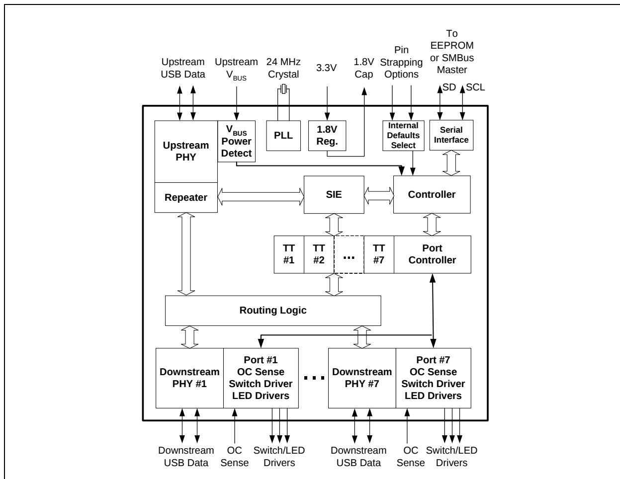
FIGURE 4-1: 7-PORT BLOCK DIAGRAM
