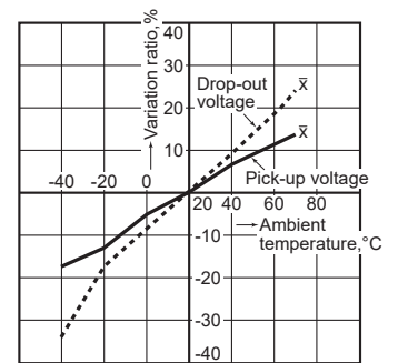
6. Ambient temperature characteristics
