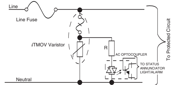
Figure 2. Application example 2
