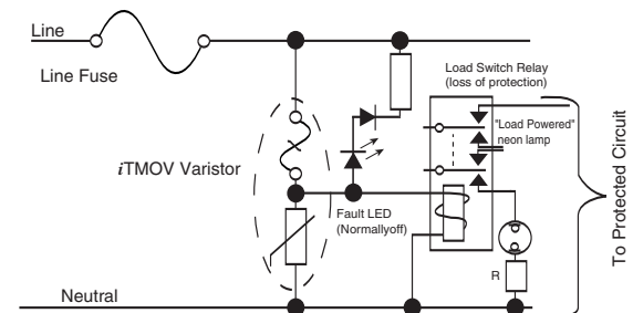
Figure 3. Application example 3
