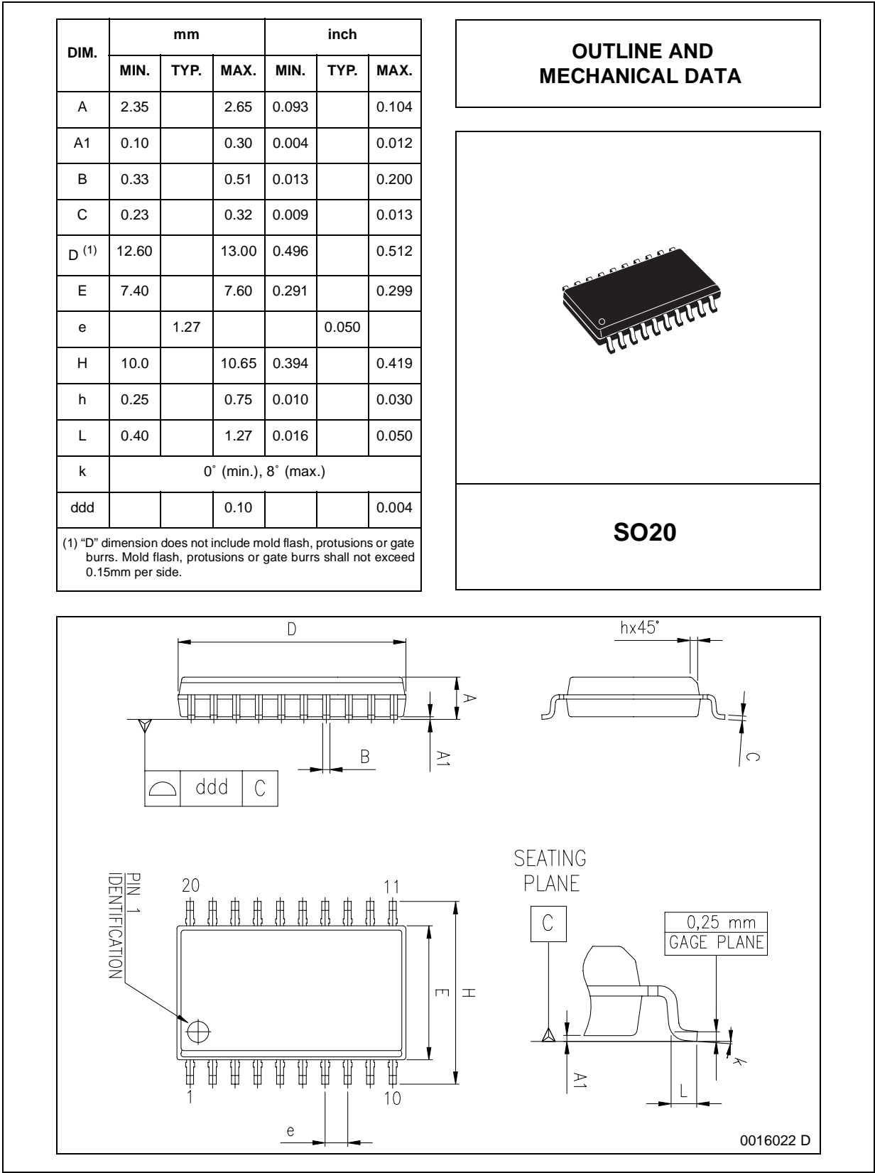
Figure 20. SO-20 Mechanical Data & Package Dimensions
