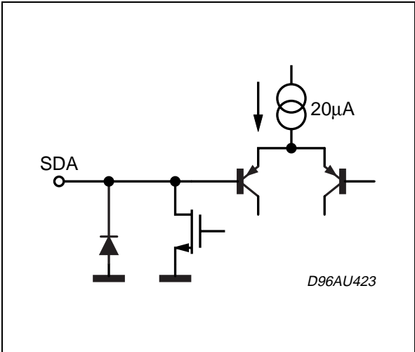
Figure 15. PINS: 9
