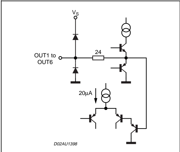
Figure 13. PINS: 2, 3, 4, 17, 18, 19
